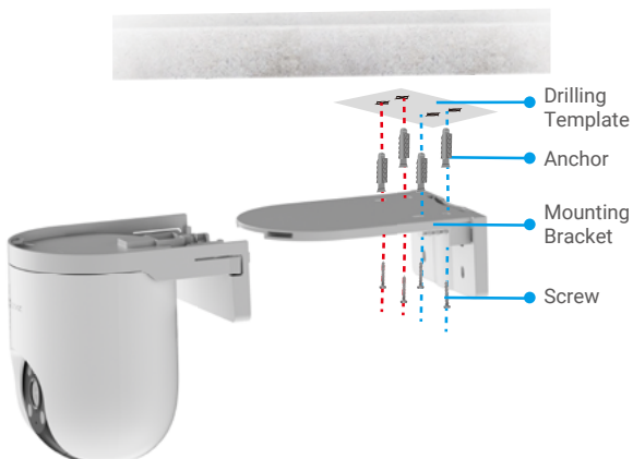
Fig. 1 Ceiling Mount
